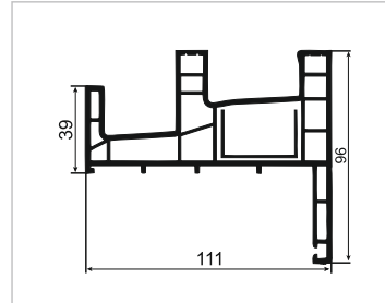
S003 Sineklikli Çiftli Pervazlı Kasa Frame Profile With Fly Screen With Sill Double Rail
