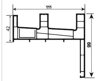
S018 Dıştan Pervazlı Sineklikli Çiftli Kasa Frame Profile Double Rail With Fly Screen From Outside
