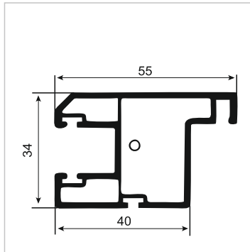
S005 Sineklik Kanat Profili New Fly Screen Sash Profile
