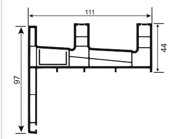
S017 İçten Pervazlı Sineklikli Çiftli Kasa Frame Profile Double Rail With Fly Screen From Inside
