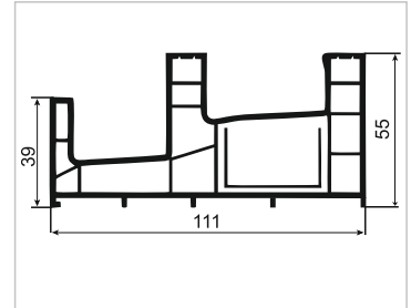
S013 Sineklikli Çiftli Kasa Frame Profile With Fly Screen Double Rail
