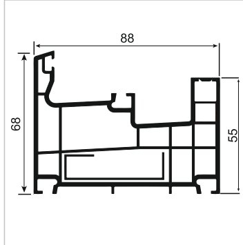
S014 Tekli Kasa Frame Profile Single Rail
