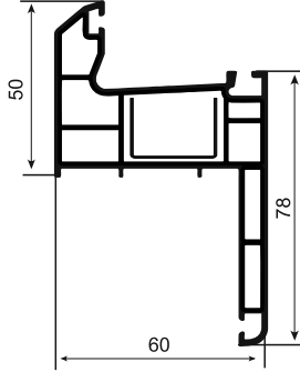
Yağ 002 Pervazlı Kasa Profili / Casing Frame Profile
