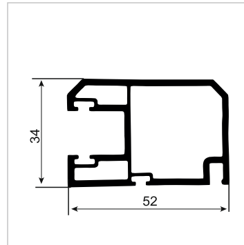
S006 Sineklik Kanat Profili Fly Screen Sash Profile
