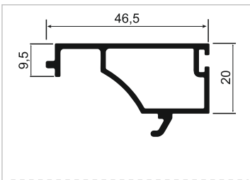
S016 Kasa Kapama Profili Sliding Frame Cover Profile
