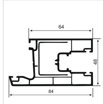
S004 Kanat Profili / Sliding Sash Profile
